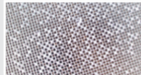
LEFT: Section of DPF showing channels blocked by lube-ash deposits from high-ash oil (white areas.)
